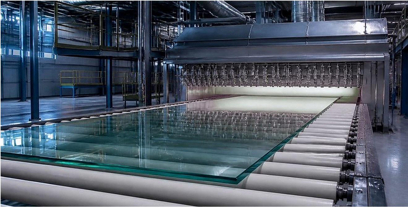
TEMPERING LINE — QUENCH SECTION
